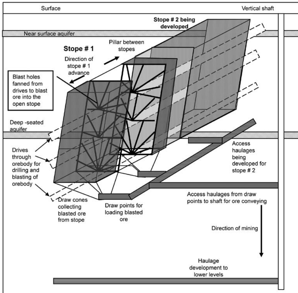
Figure 5.8: Isometric view through a massive orebody employing sub-level opening stope mining method
