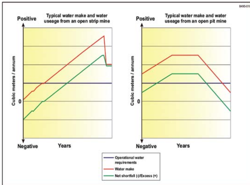
Figure 5-2: Typical water make and water use for opencast mines
