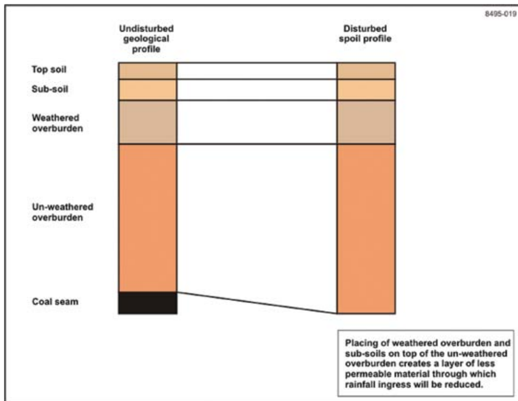
Figure 6-35: Best practice for spoils placement to reduce rainfall ingress
