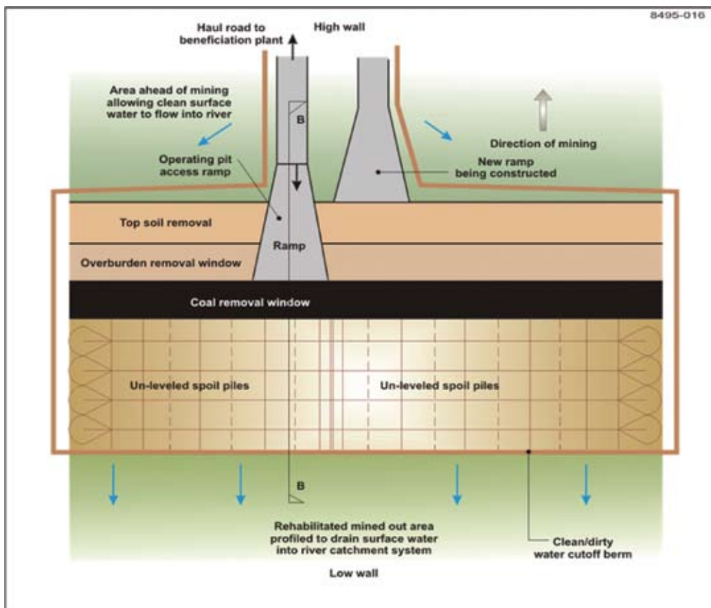
Figure 6-33: Plan view of best practices utilising high wall ramps
