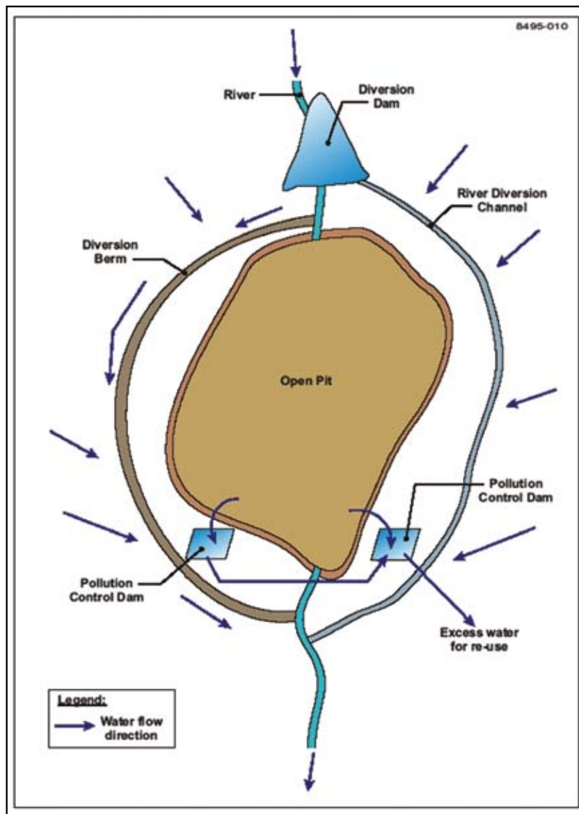
Figure 6-17: Typical water management measures for mining in a watercourse
