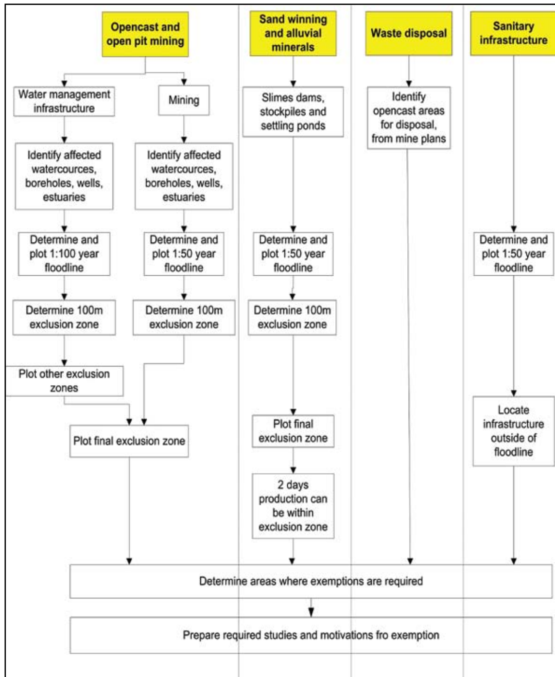
Figure 6-16: Process for siting water management facilities
