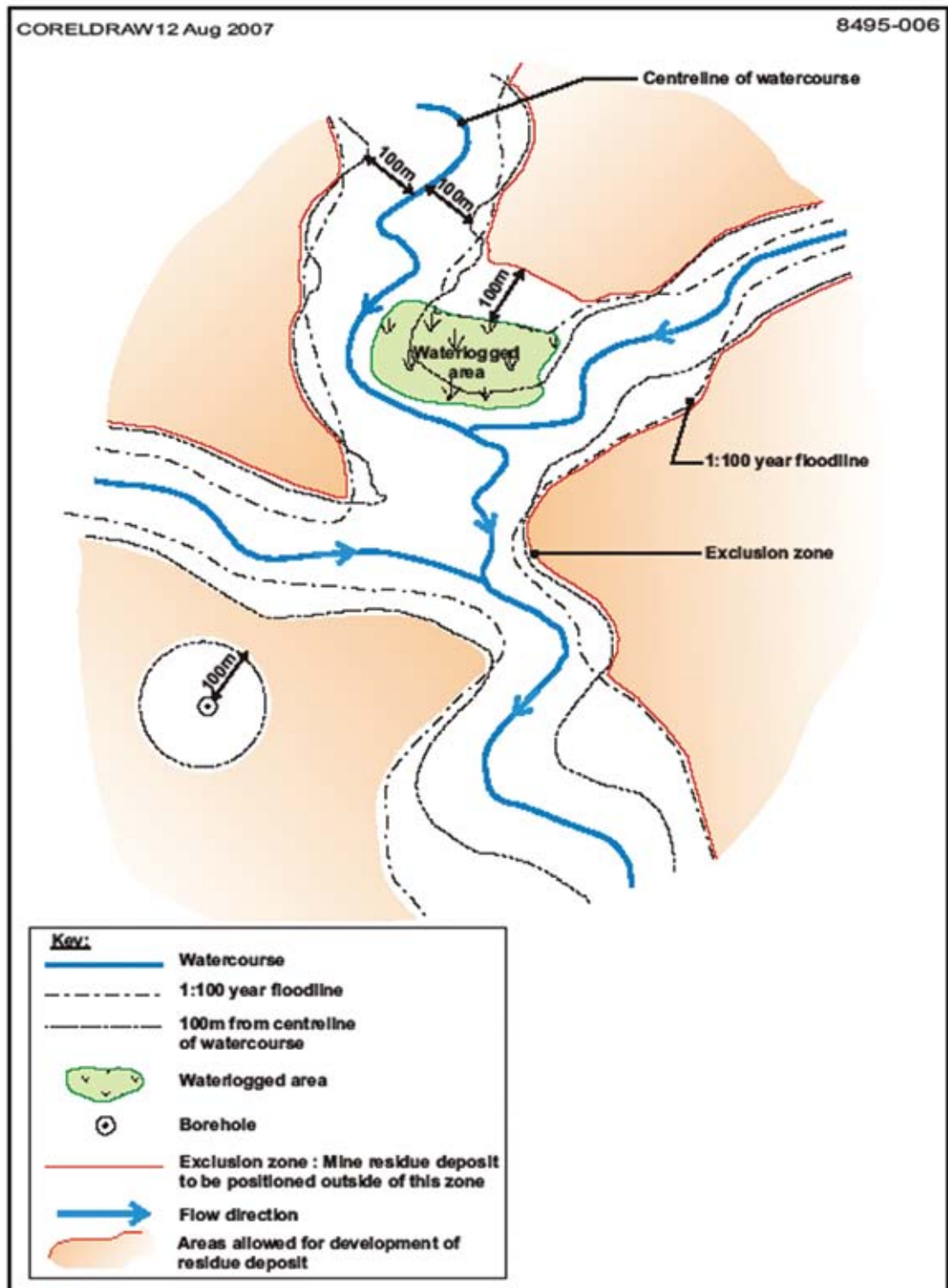
Figure 6-18: Siting of a mine residue deposit
