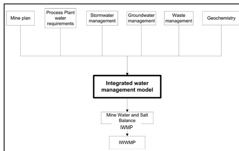
Figure 6-1: Integrated water management modelling for a surface mine
