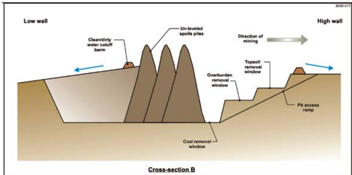
Figure 6-34: Section through mine pit with high wall ramps
