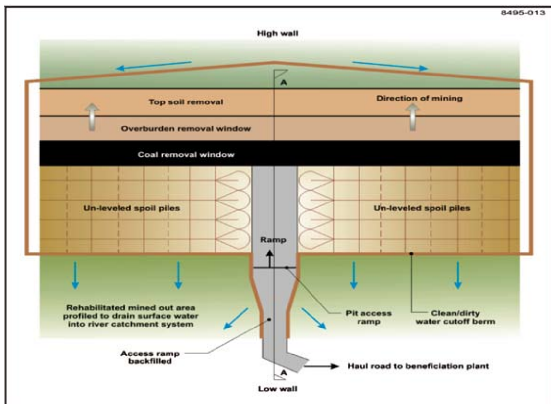
Figure 6-31: Plan view of best practices utilising low wall ramps
