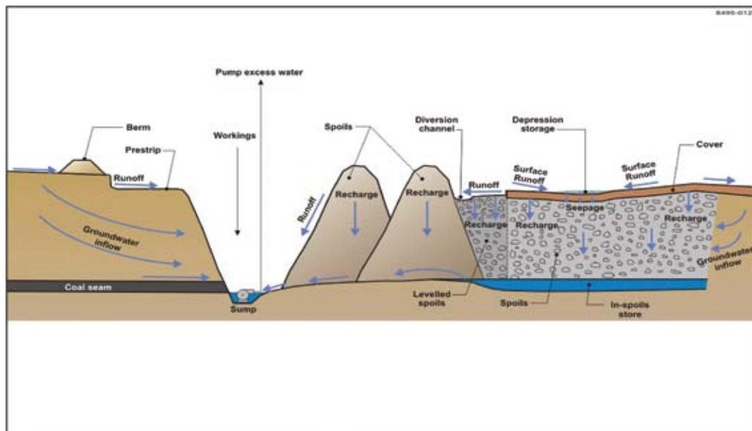
Figure 6-2: Typical water flow paths in an open pit mine
